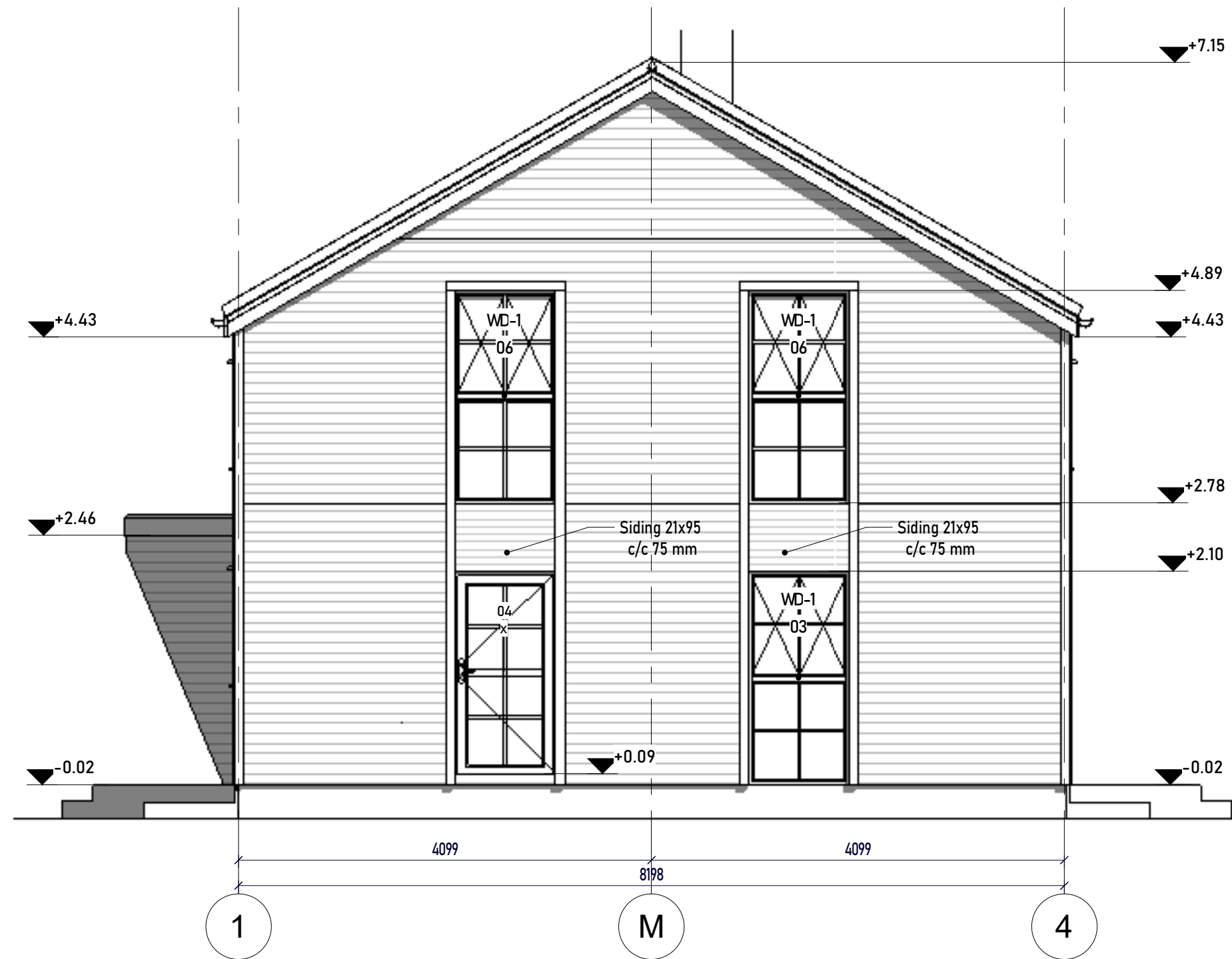
1 Facade 1-4 - North 1:50
